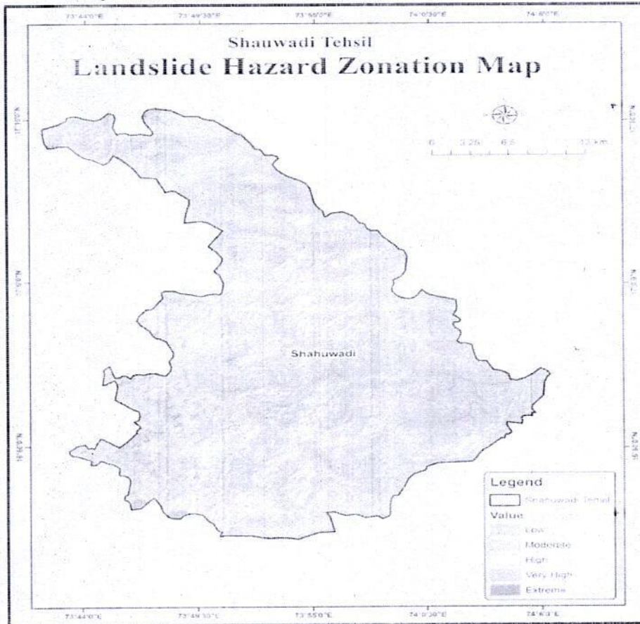
Map. No. 3 Shahuwadi Tehsil: Landslide Hazard Map
